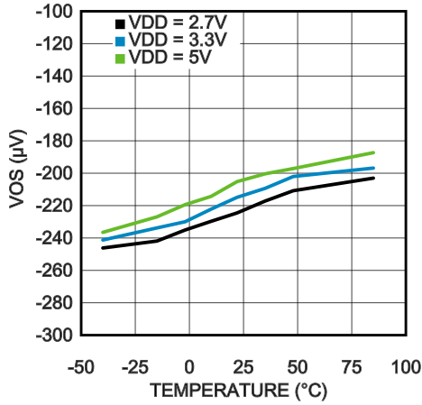
Input V OS_RW vs. temperature (V bias 0mV)
